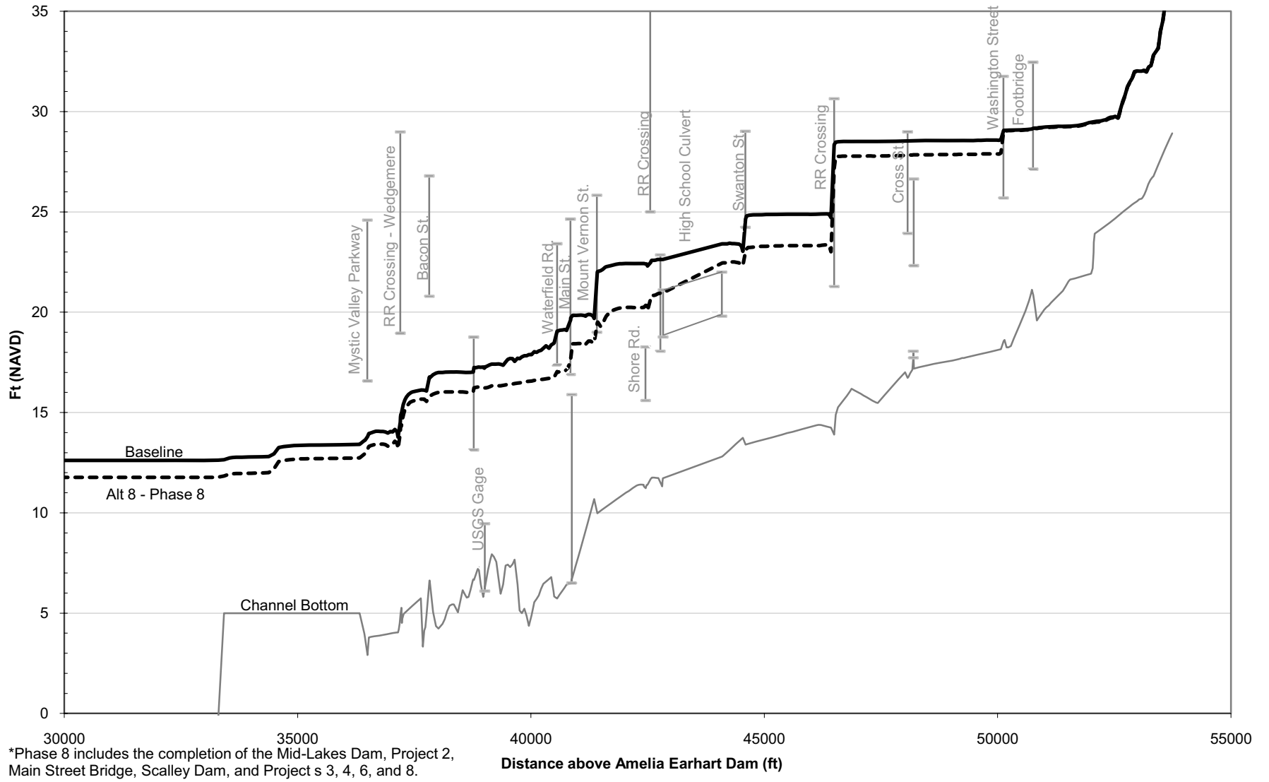
Figure M-29: 100-Year Flood Profile, Alt. 8 Phase 8* vs. Baseline (No Action) Conditions
