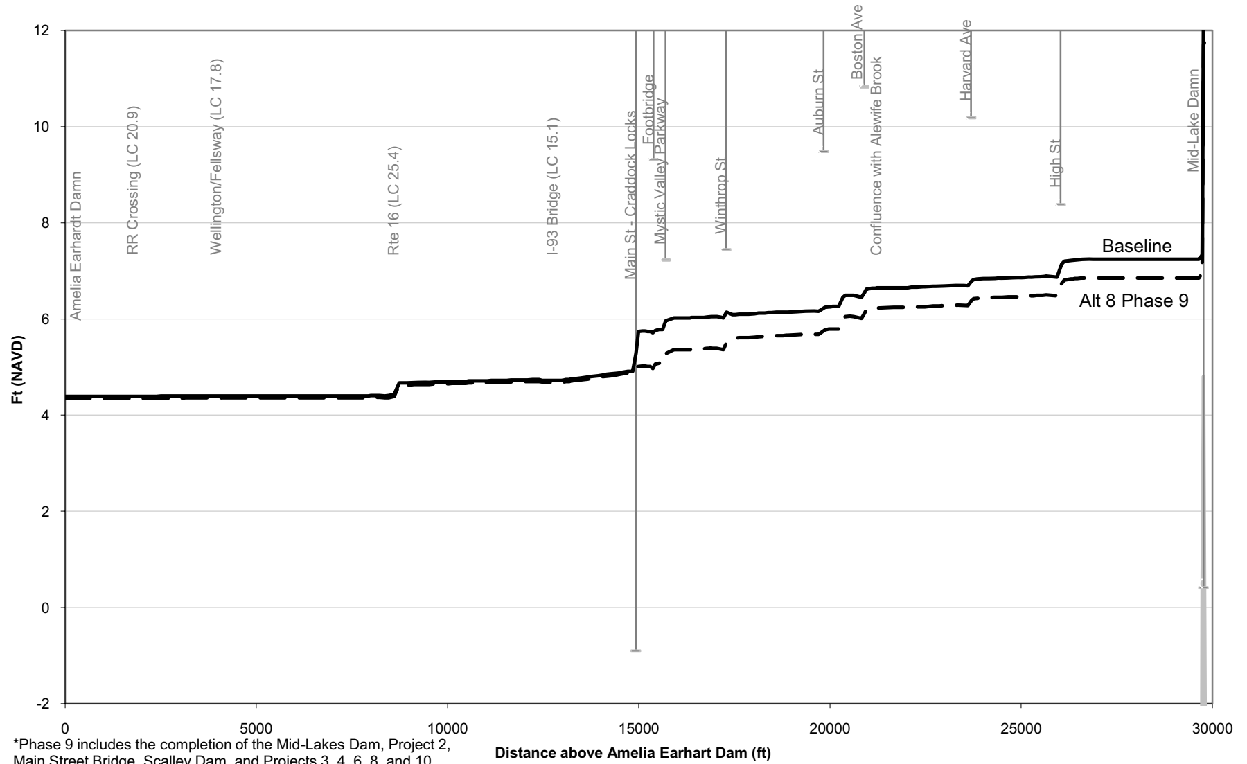
Figure M-33: 100-Year Flood Profile, Alt. 8 Phase 9* vs. Baseline (No Action) Conditions
