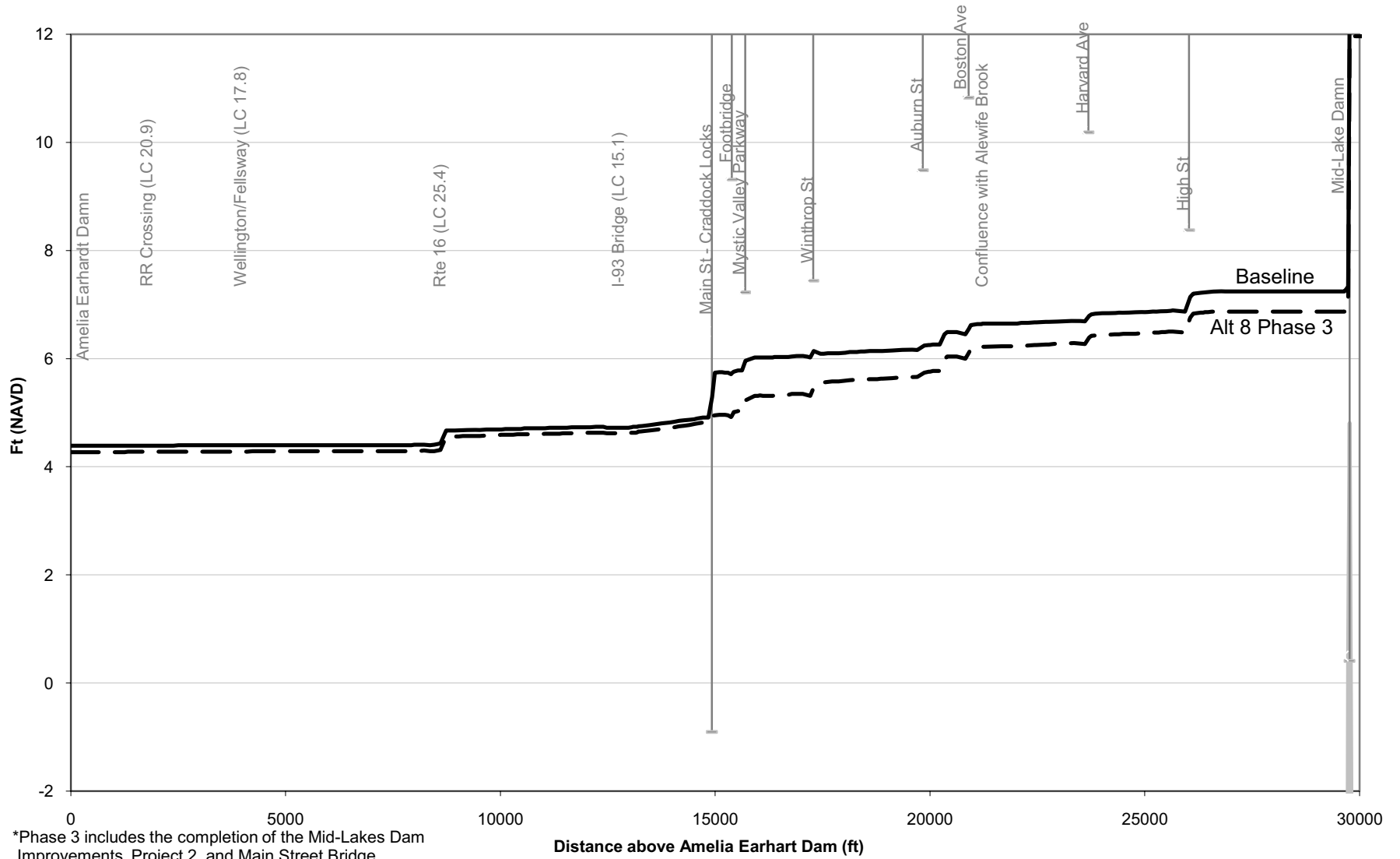
Figure M-15: 100-Year Flood Profile, Alt. 8 Phase 3* vs. Baseline (No Action) Conditions
