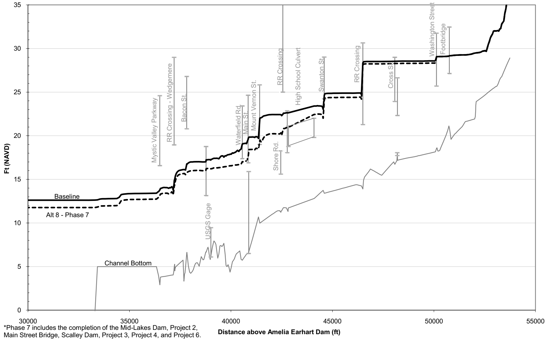
Figure M-26: 100-Year Flood Profile, Alt. 8 Phase 7* vs. Baseline (No Action) Conditions
