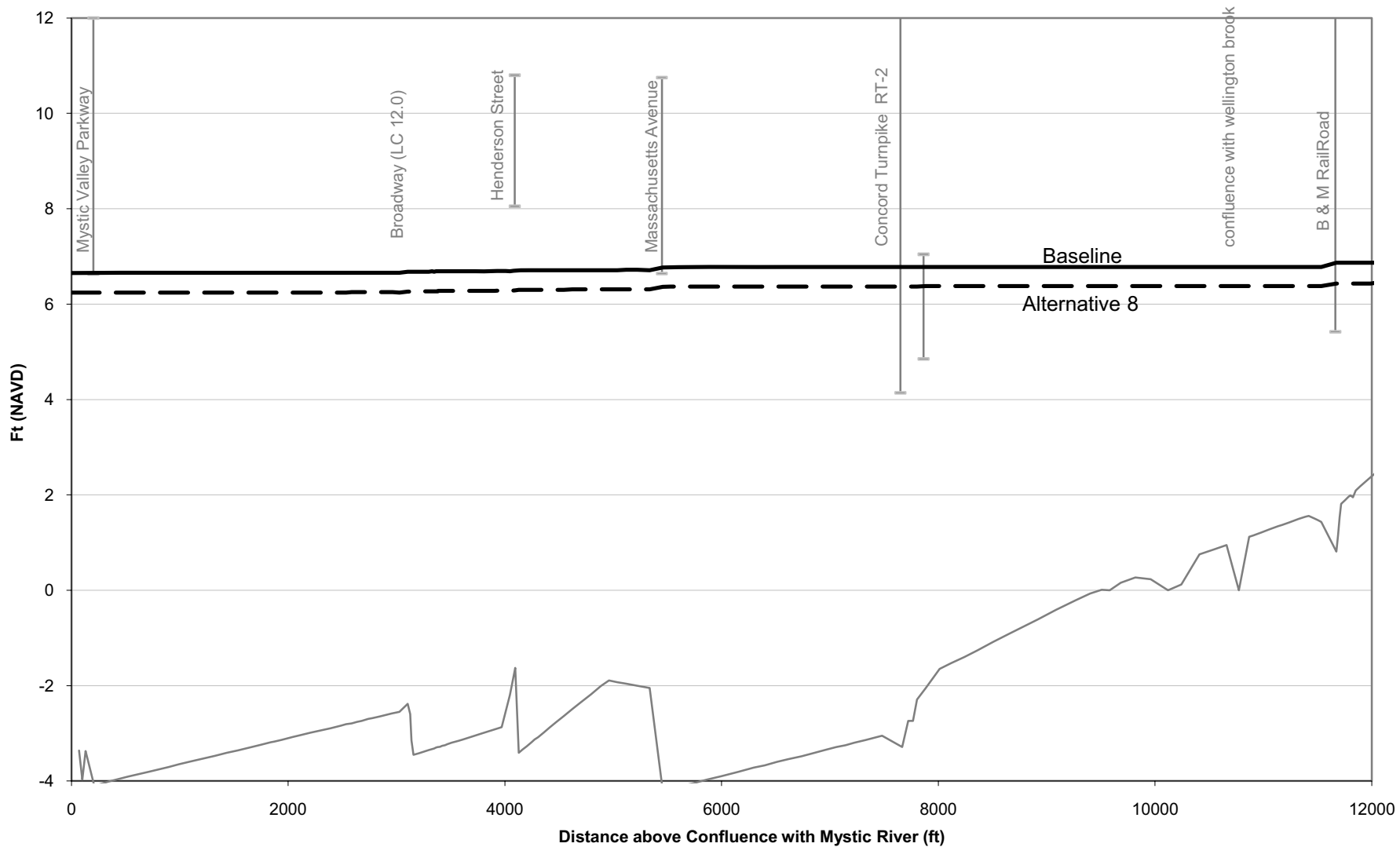
Figure M-4: 100-Year Flood Profile, Alternative 8 vs. Baseline (No Action) Conditions
