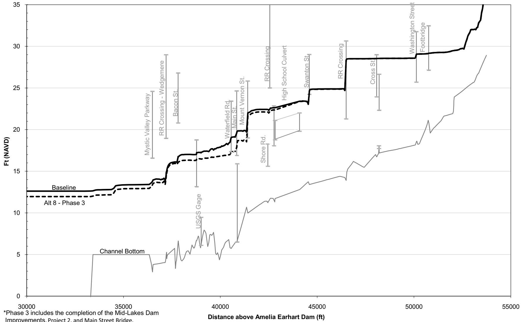
Figure M-14: 100-Year Flood Profile, Alt. 8 Phase 3* vs. Baseline (No Action) Conditions
