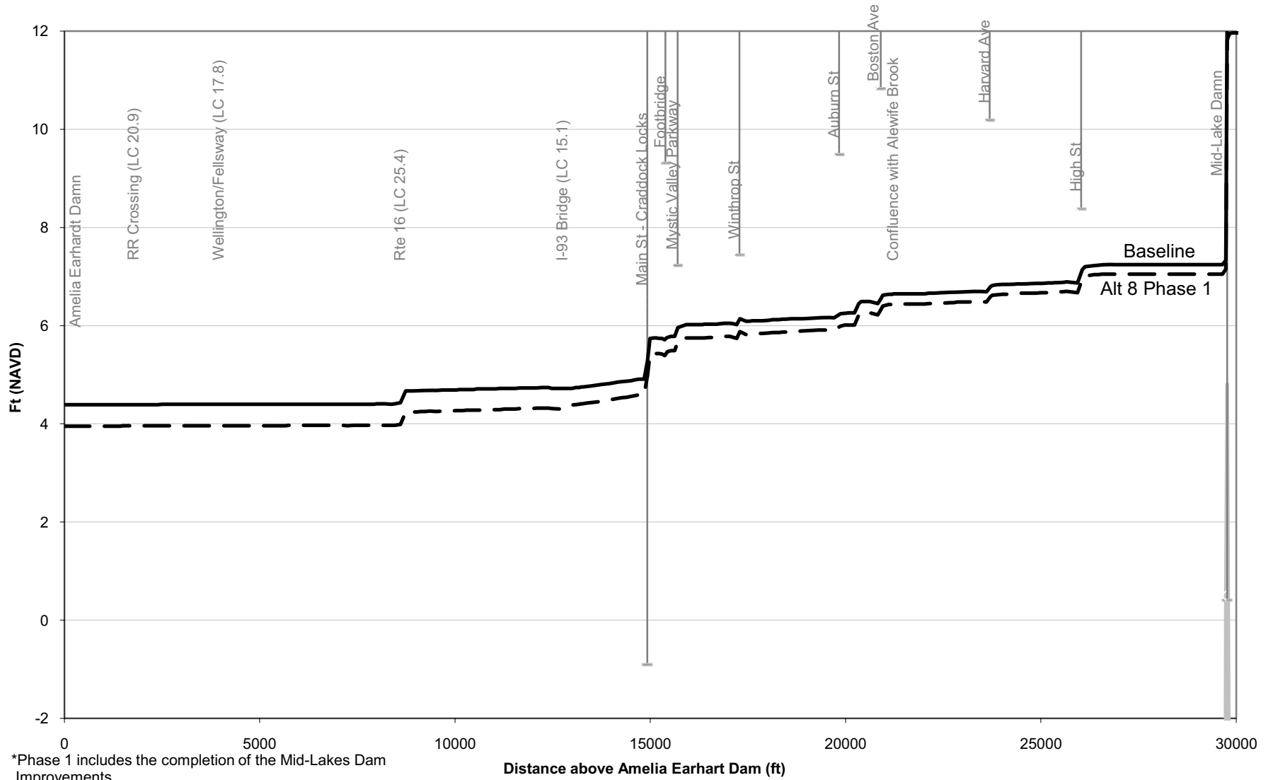
Figure M-9: 100-Year Flood Profile, Alt. 8 Phase 1* vs. Baseline (No Action) Conditions
