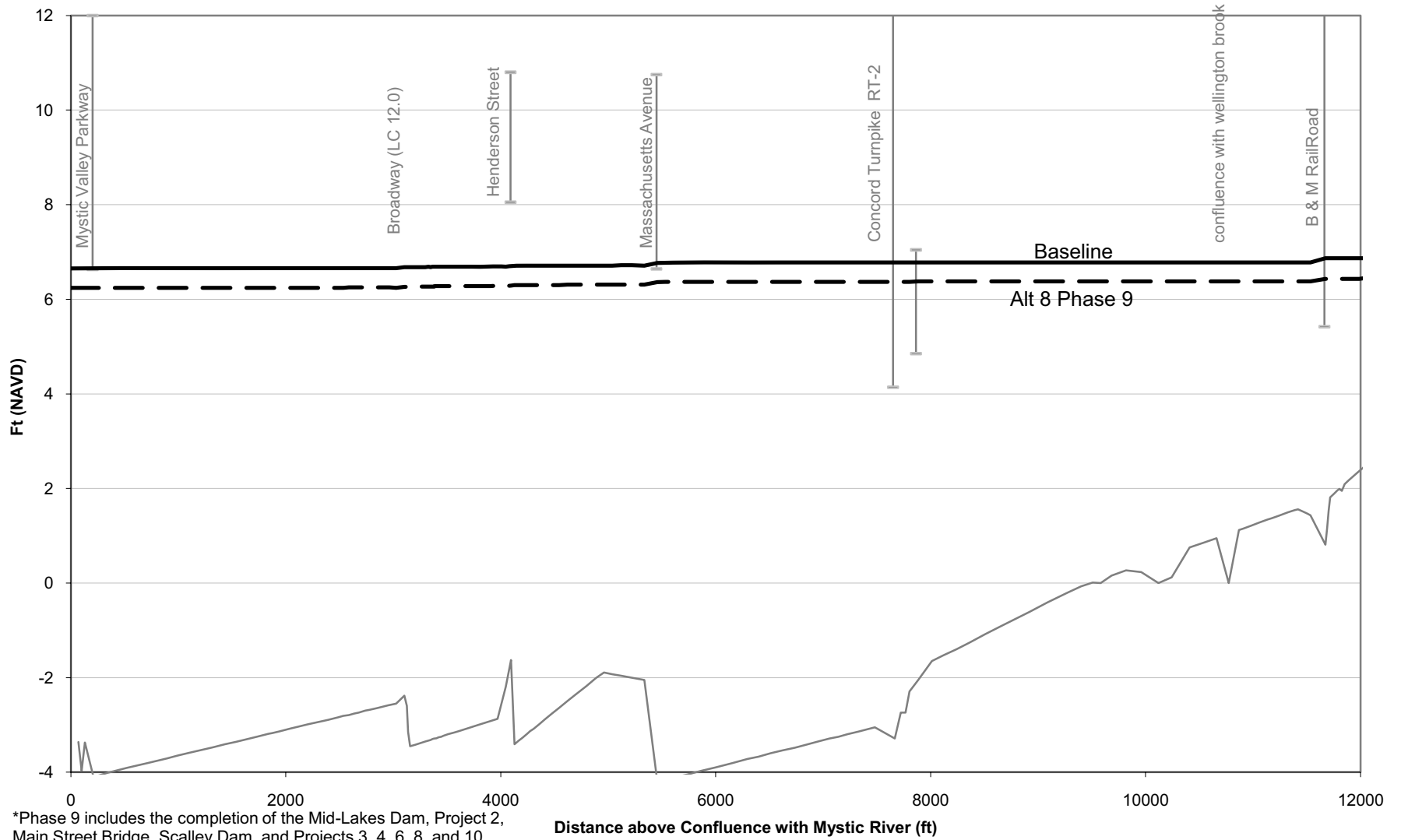
Figure M-34: 100-Year Flood Profile, Alt. 8 Phase 9* vs. Baseline (No Action) Conditions
