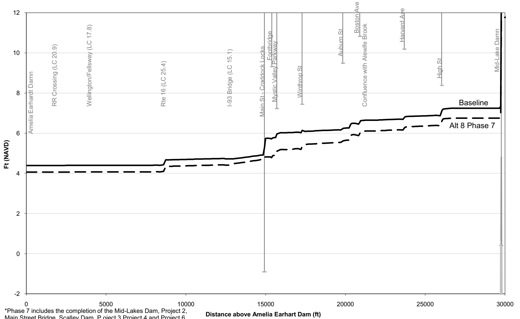
Figure M-27: 100-Year Flood Profile, Alt. 8 Phase 7* vs. Baseline (No Action) Conditions
