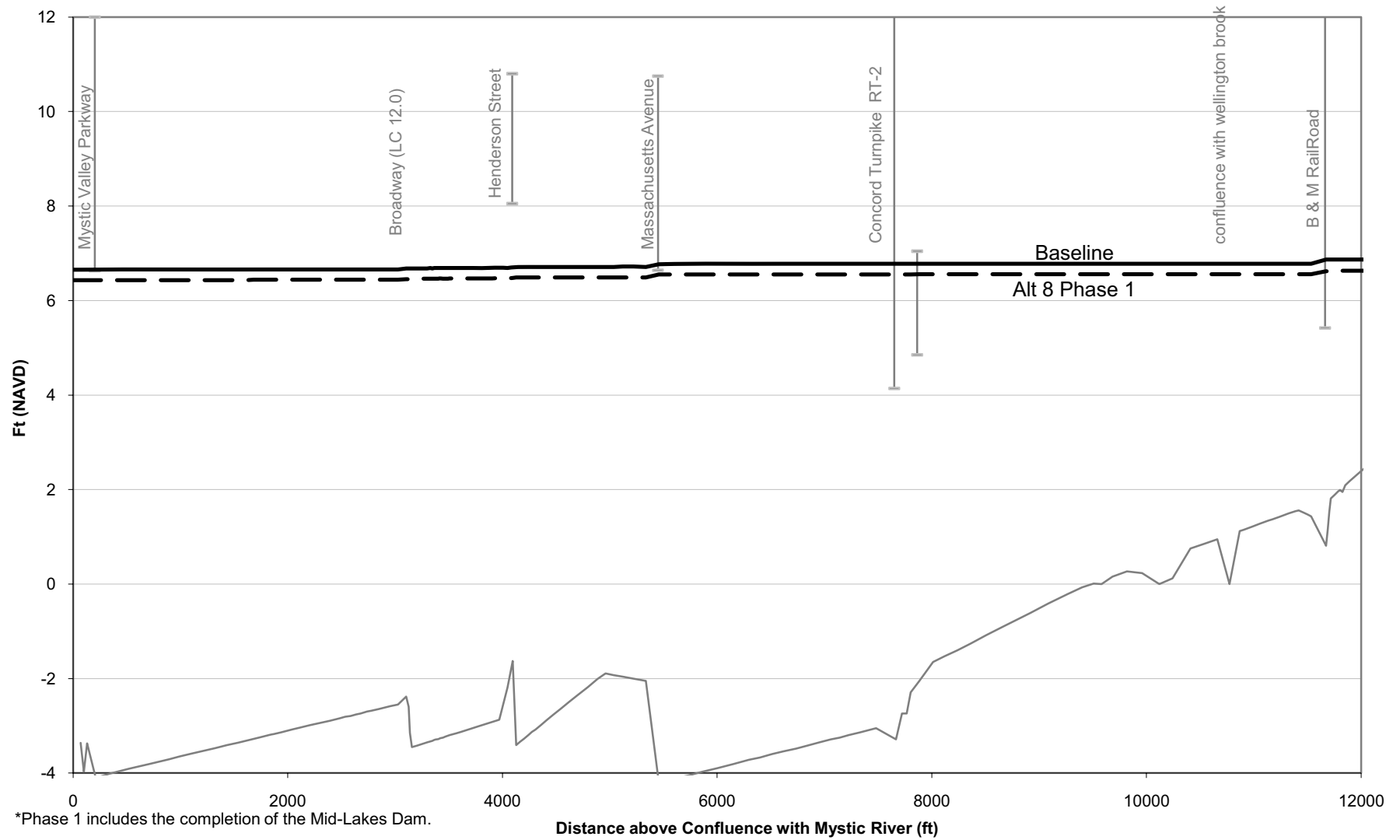
Figure M-10: 100-Year Flood Profile, Alt. 8 Phase 1* vs. Baseline (No Action) Conditions
