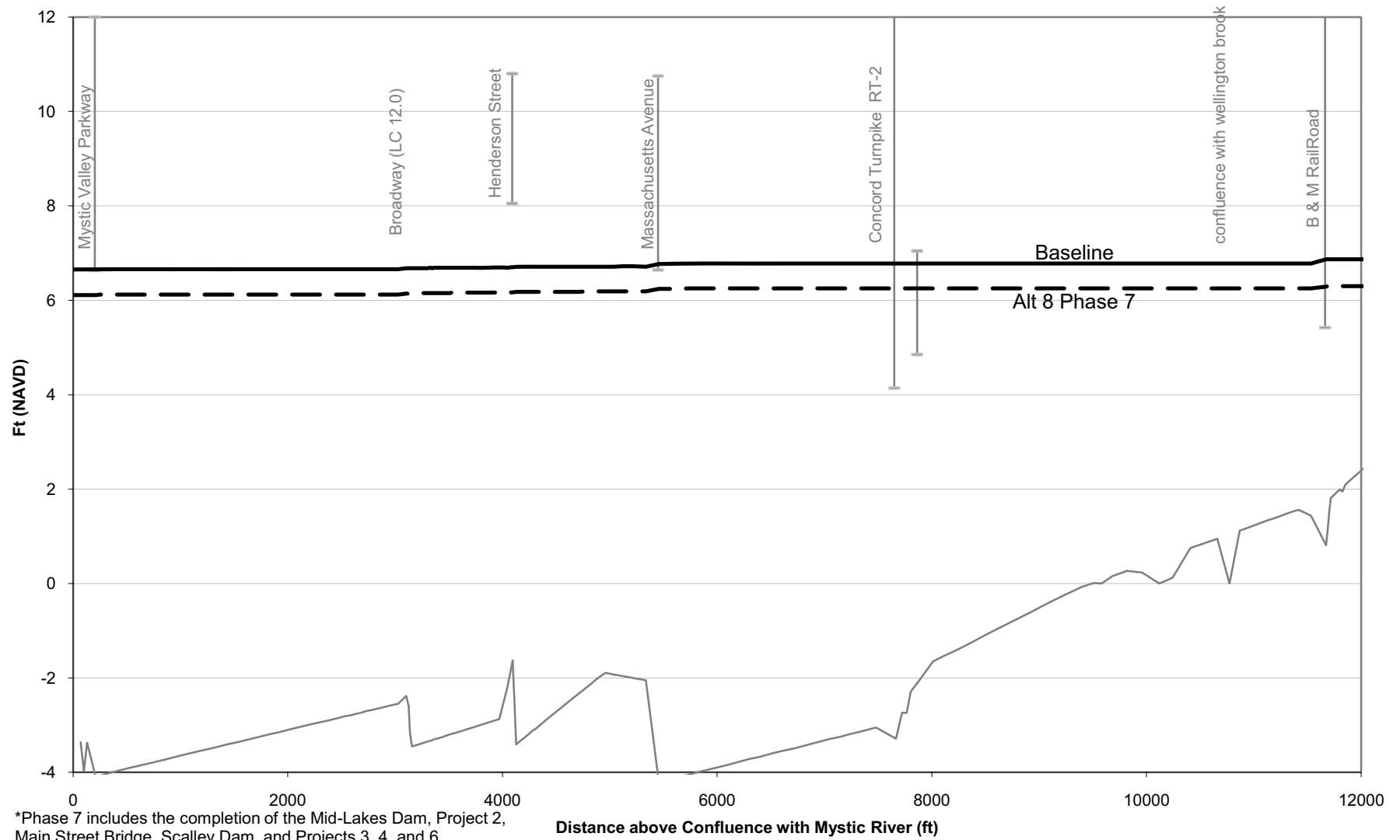
Figure M-28: 100-Year Flood Profile, Alt. 8 Phase 7* vs. Baseline (No Action) Conditions
