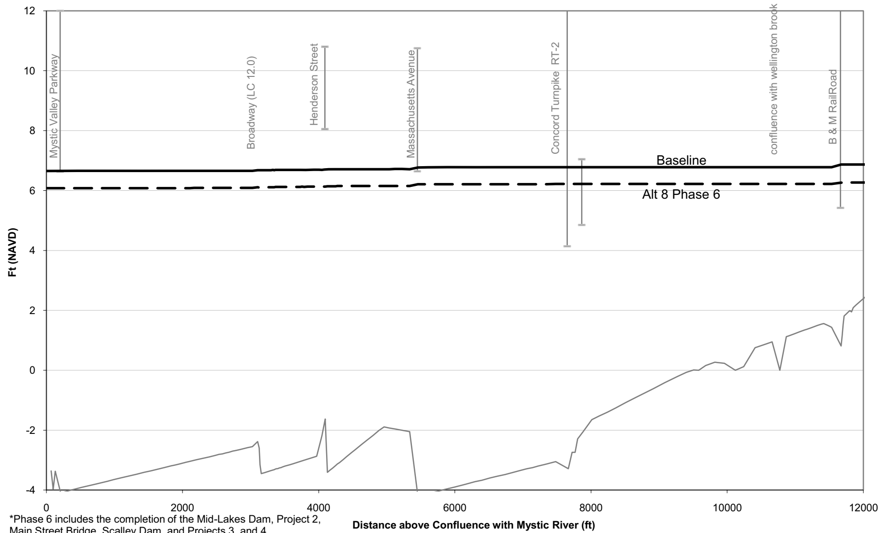
Figure M-25: 100-Year Flood Profile, Alt. 8 Phase 6* vs. Baseline (No Action) Conditions
