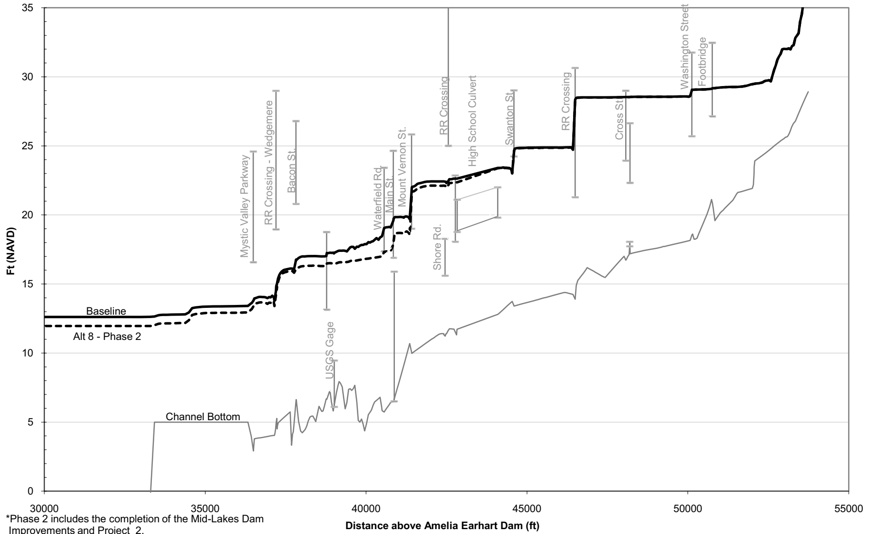
Figure M-11: 100-Year Flood Profile, Alt. 8 Phase 2* vs. Baseline (No Action) Conditions
