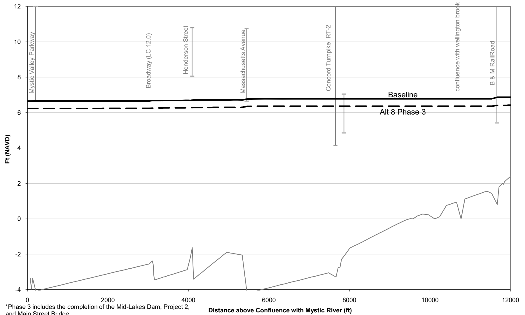
Figure M-16: 100-Year Flood Profile, Alt. 8 Phase 3* vs. Baseline (No Action) Conditions
