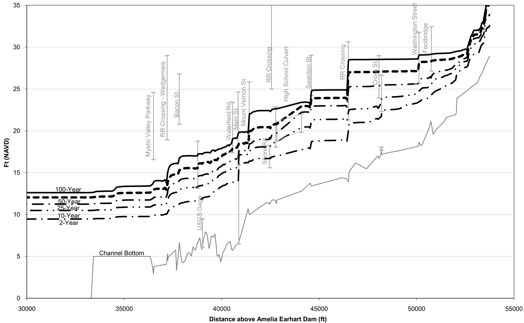
Figure M-1: 2, 10, 25, 50 & 100-Year Flood Profile, Existing (No Action) Conditions
