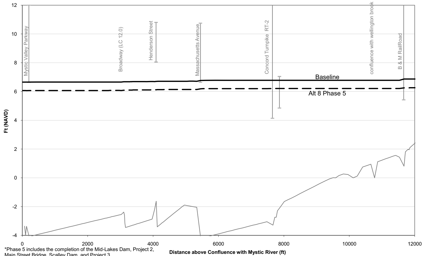
Figure M-22: 100-Year Flood Profile, Alt. 8 Phase 5* vs. Baseline (No Action) Conditions
