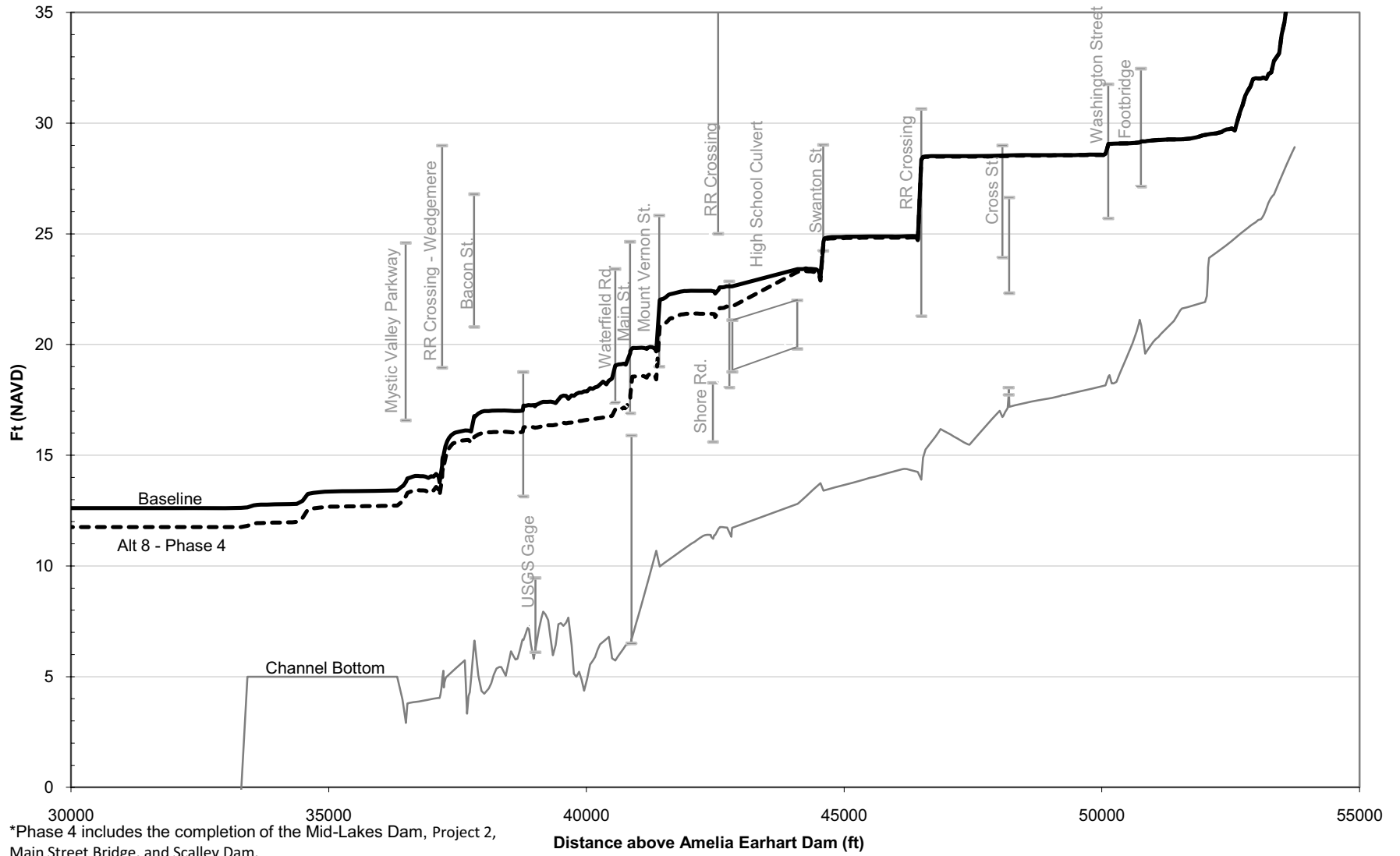
Figure M-17: 100-Year Flood Profile, Alt. 8 Phase 4* vs. Baseline (No Action) Conditions
