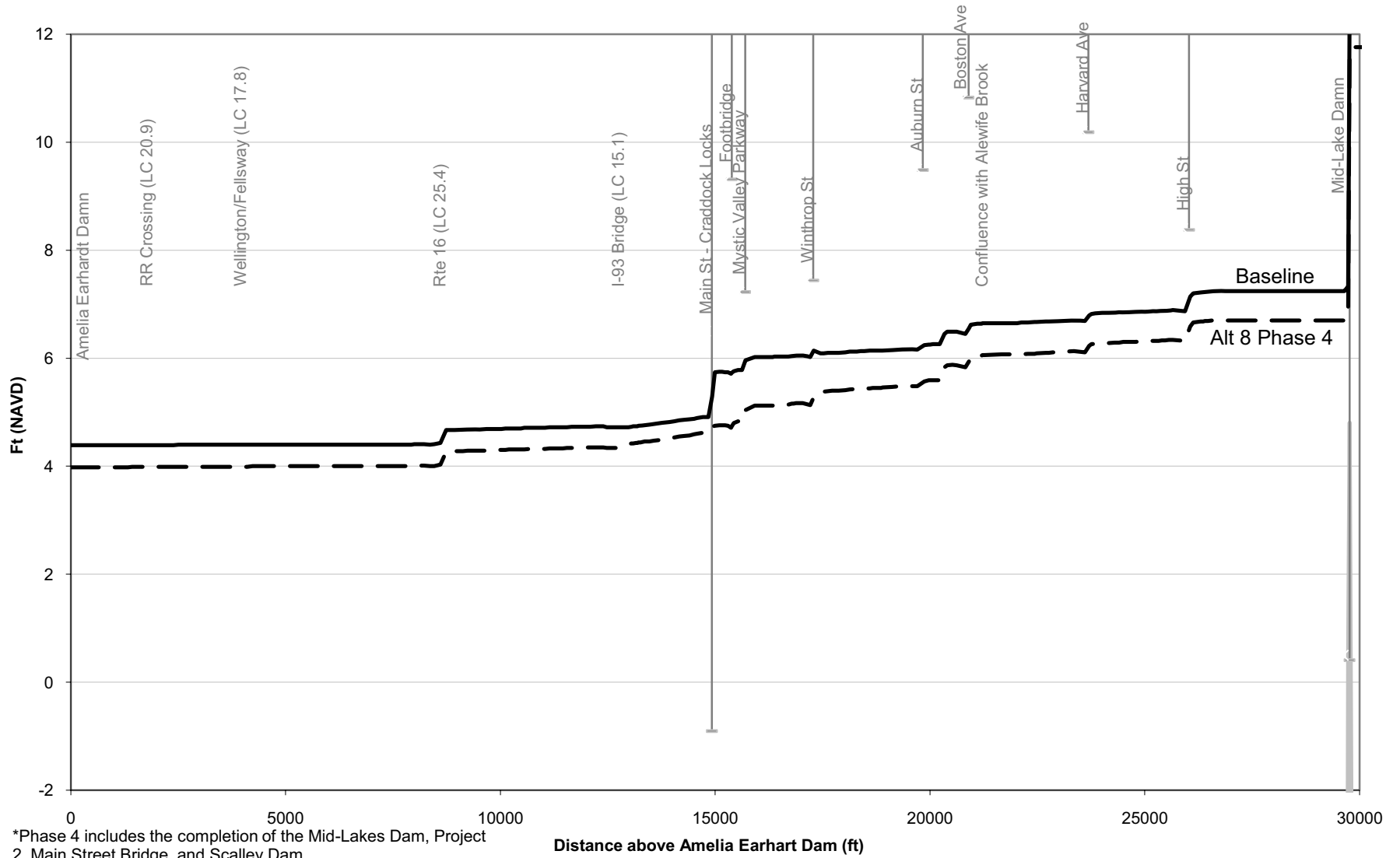
Figure M-18: 100-Year Flood Profile, Alt. 8 Phase 4* vs. Baseline (No Action) Conditions
