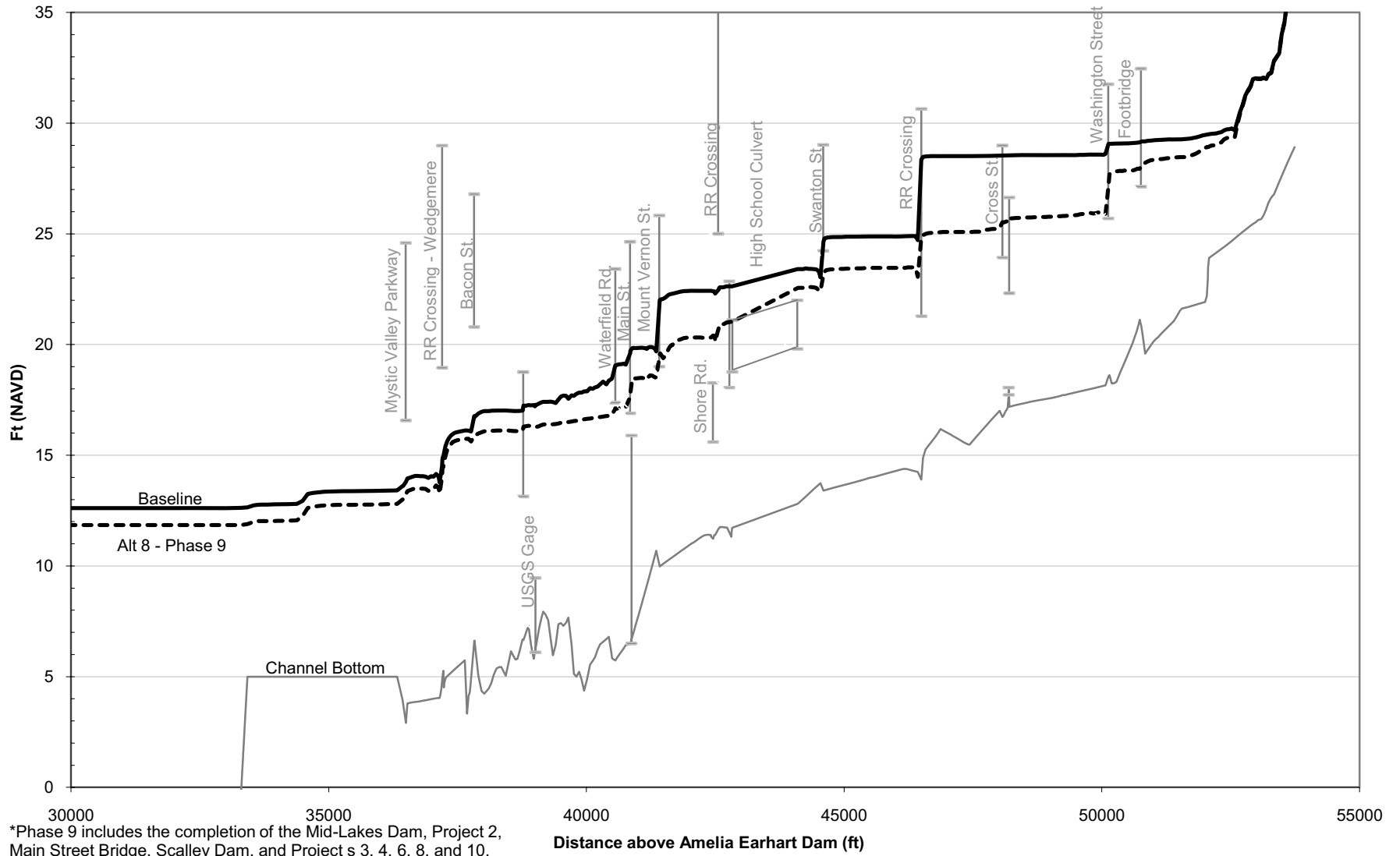
Figure M-32: 100-Year Flood Profile, Alt. 8 Phase 9* vs. Baseline (No Action) Conditions
