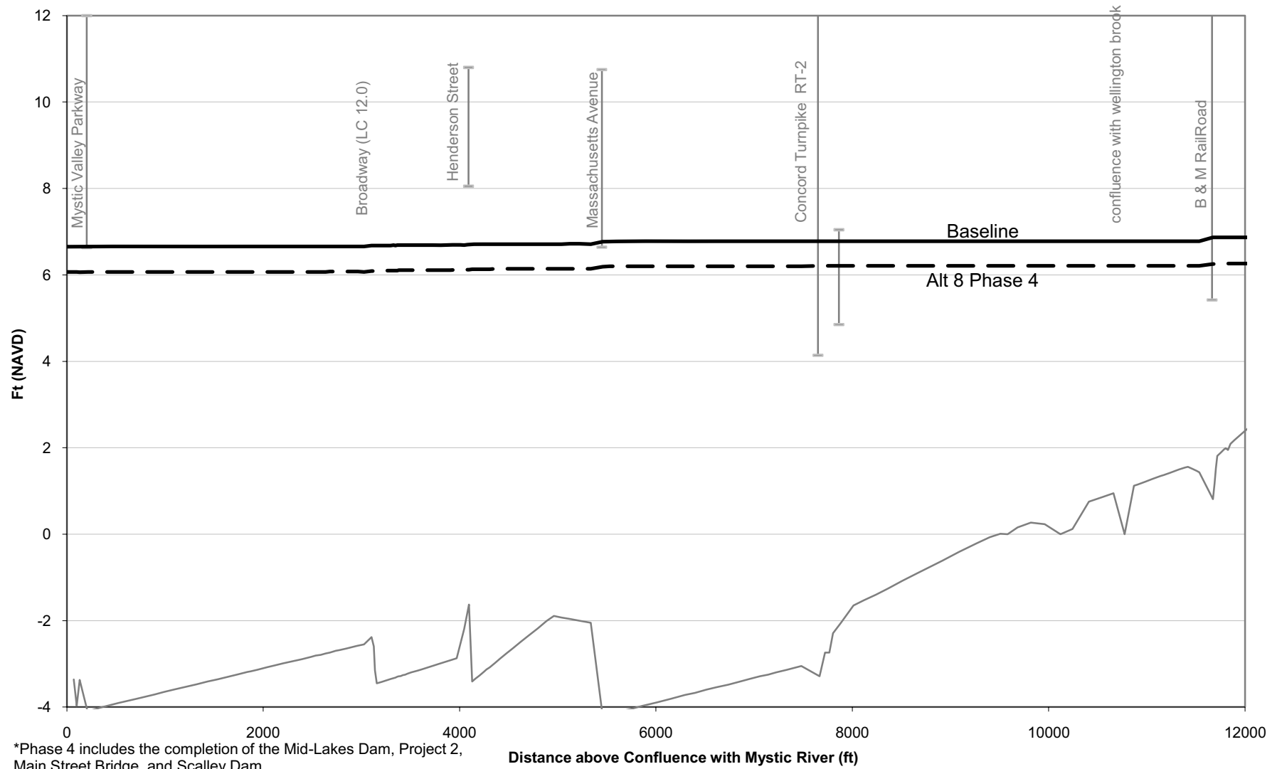
Figure M-19: 100-Year Flood Profile, Alt. 8 Phase 4* vs. Baseline (No Action) Conditions
