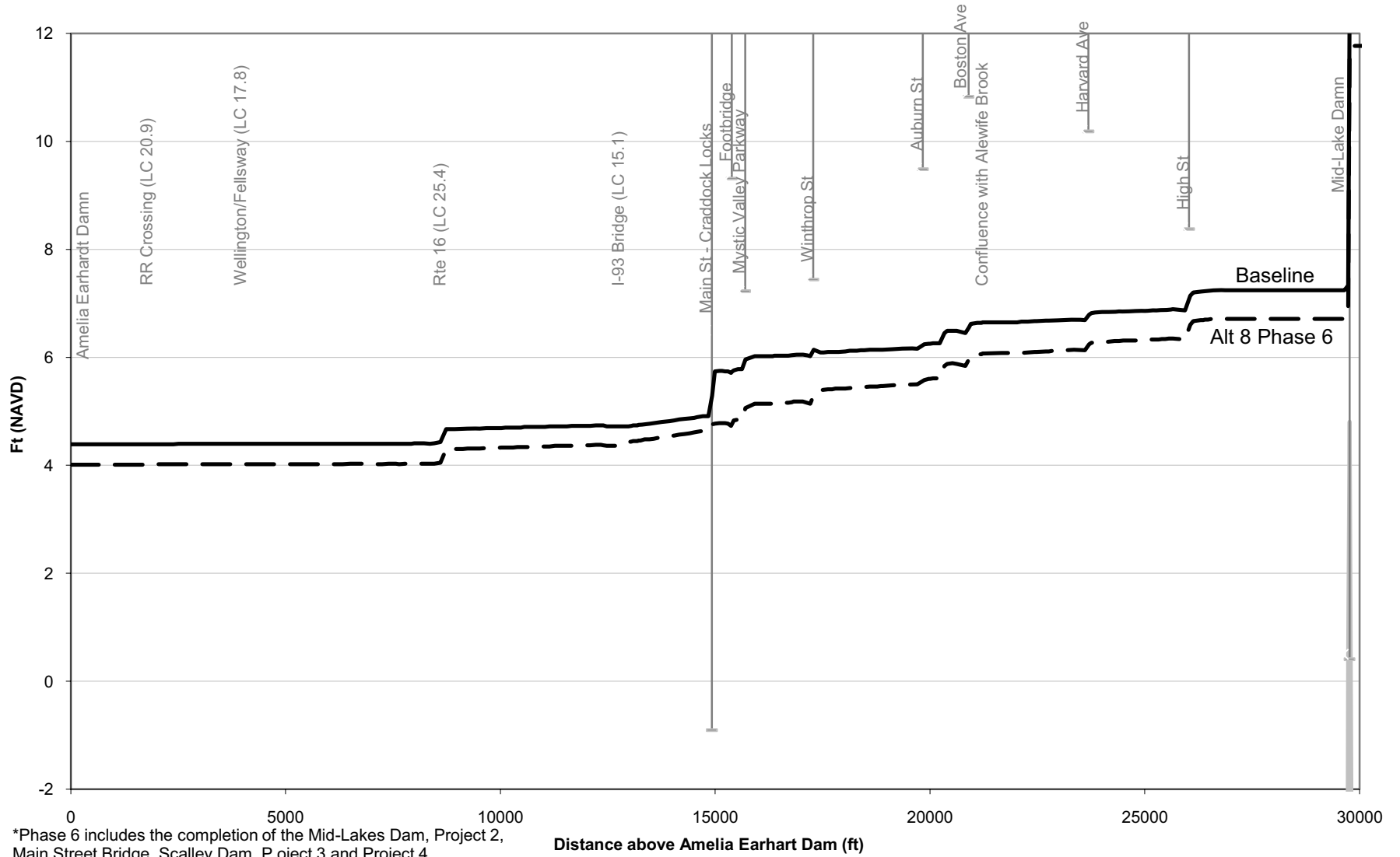
Figure M-24: 100-Year Flood Profile, Alt. 8 Phase 6* vs. Baseline (No Action) Conditions
