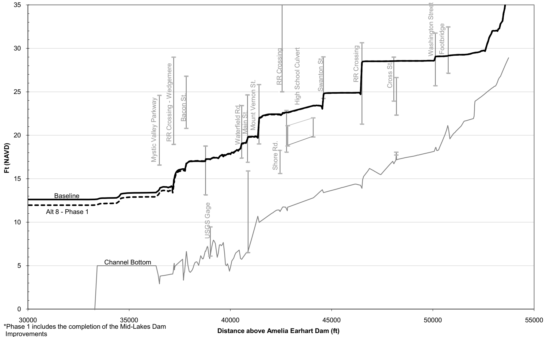
Figure M-8: 100-Year Flood Profile, Alt. 8 Phase 1* vs. Baseline (No Action) Conditions
