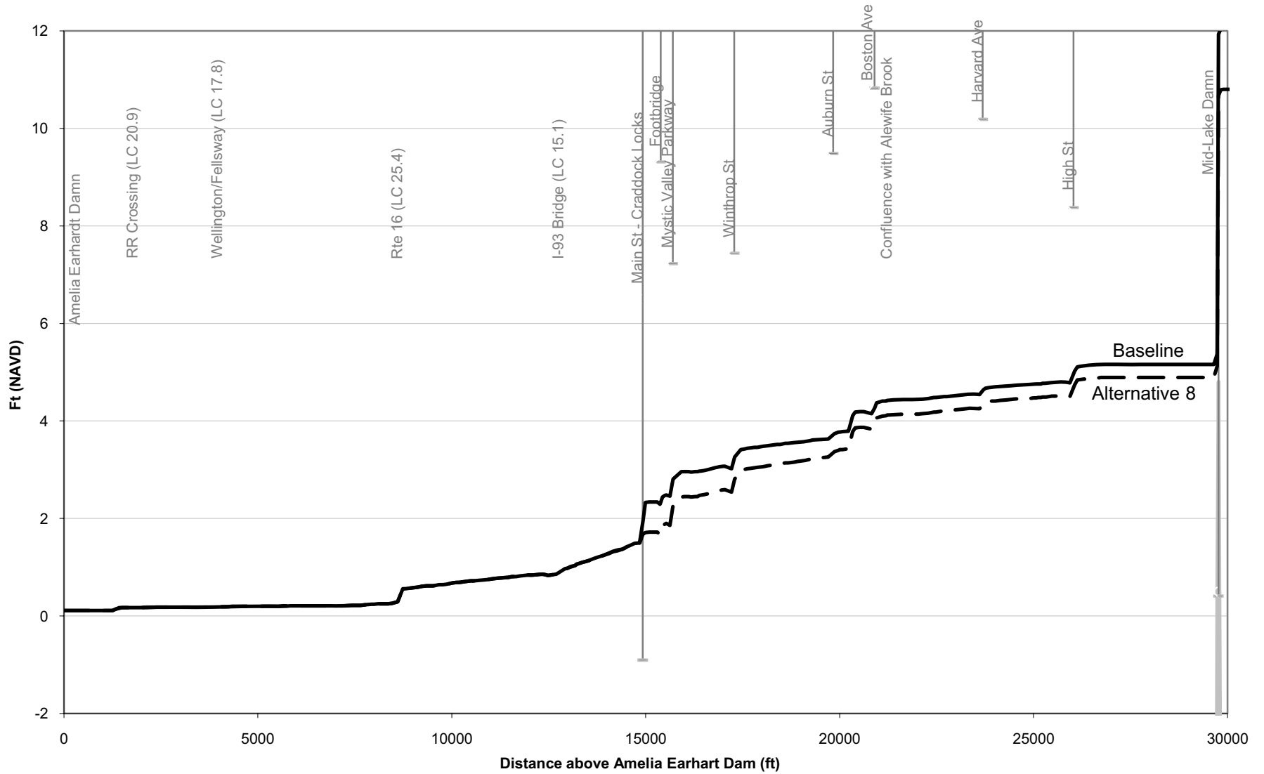
Figure M-6: 50-Year Flood Profile, Alternative 8 vs. Baseline (No Action) Conditions
