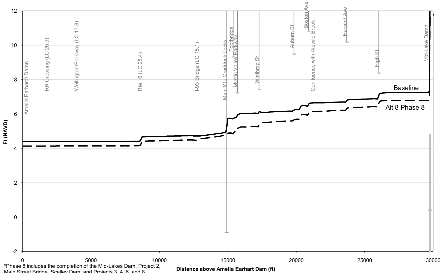
Figure M-30: 100-Year Flood Profile, Alt. 8 Phase 8* vs. Baseline (No Action) Conditions
