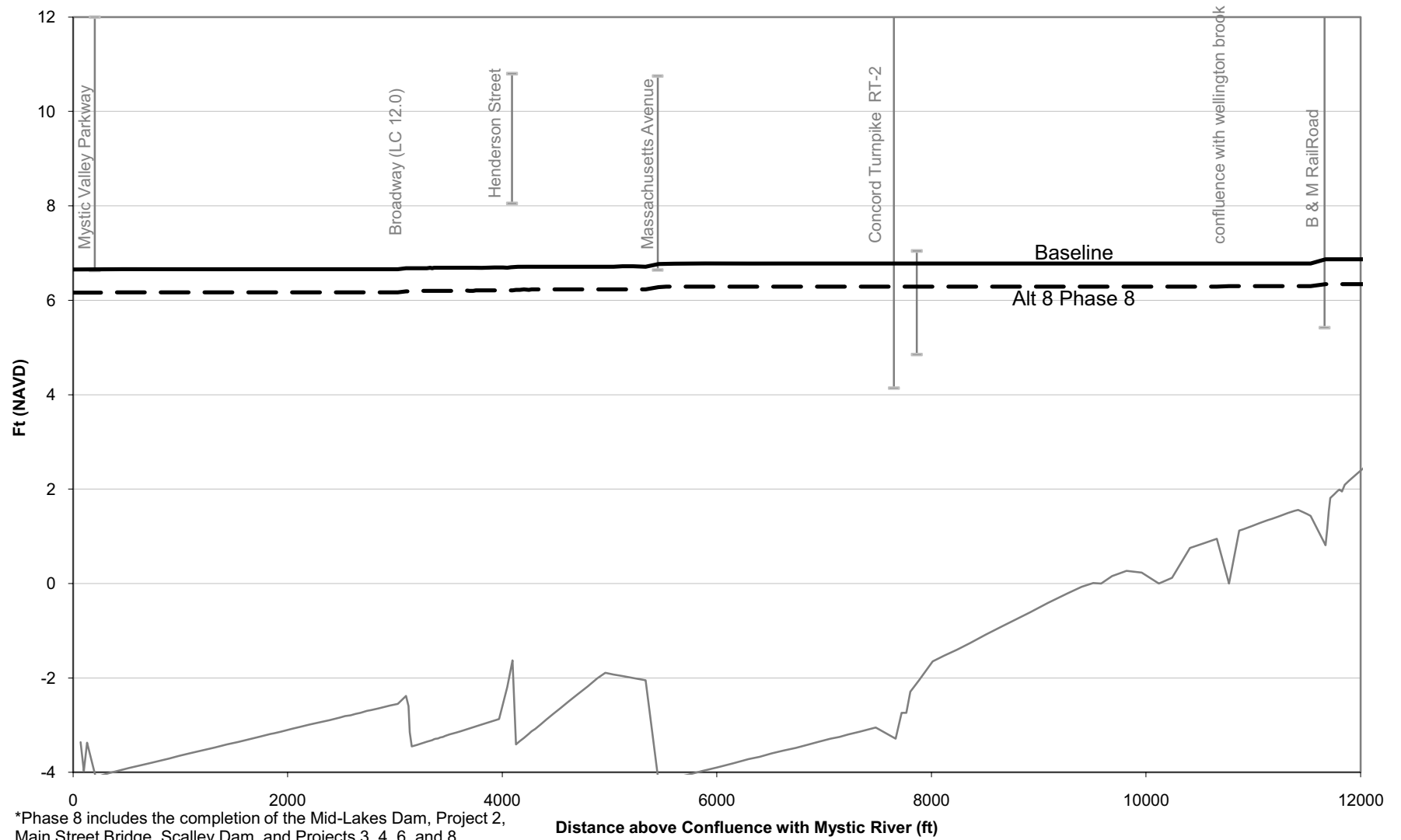
Figure M-31: 100-Year Flood Profile, Alt. 8 Phase 8* vs. Baseline (No Action) Conditions
