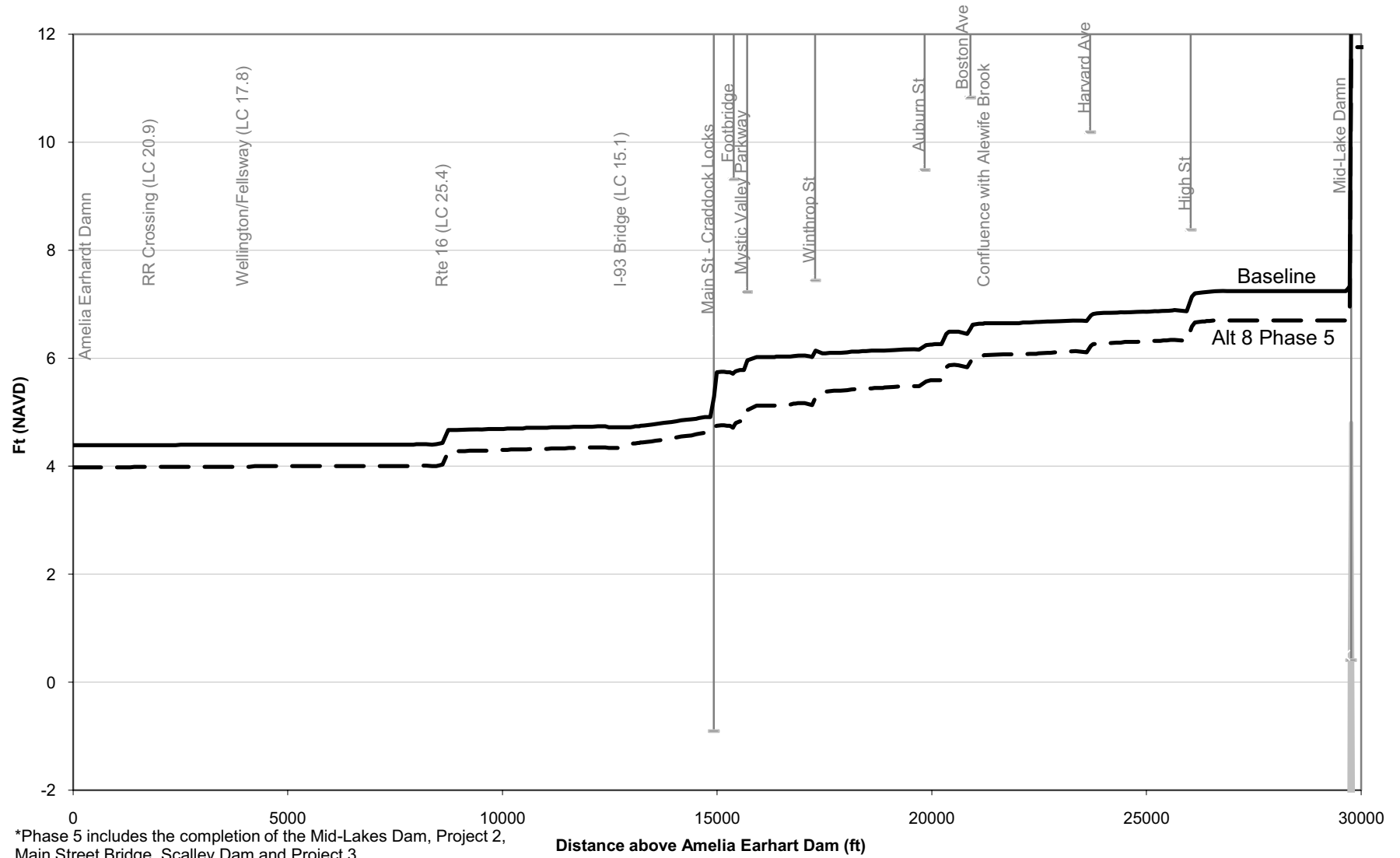
Figure M-21: 100-Year Flood Profile, Alt. 8 Phase 5* vs. Baseline (No Action) Conditions
