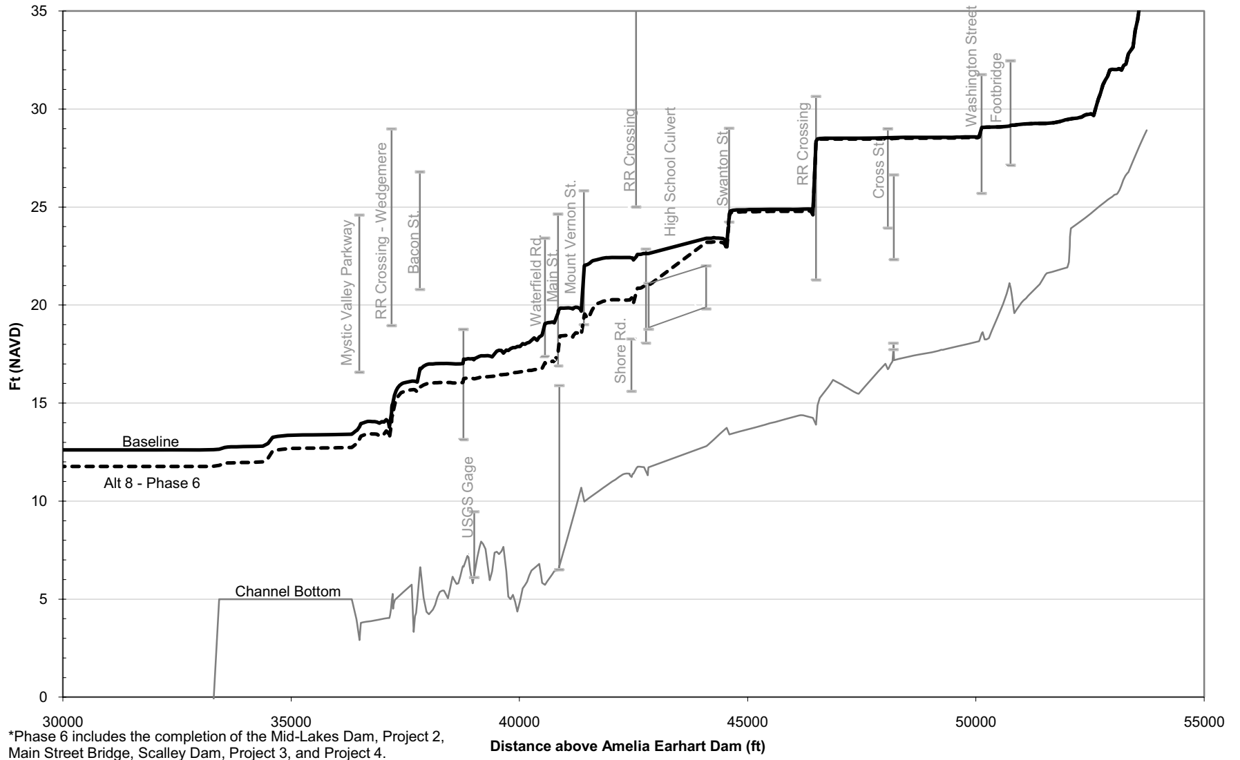
Figure M-23: 100-Year Flood Profile, Alt. 8 Phase 6* vs. Baseline (No Action) Conditions
