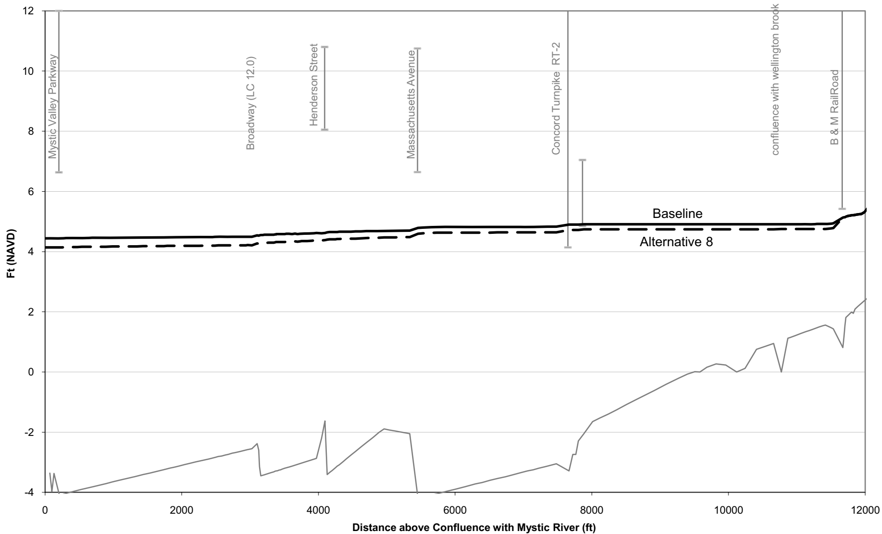
Figure M-7: 50-Year Flood Profile, Alternative 8 vs. Baseline (No Action) Conditions
