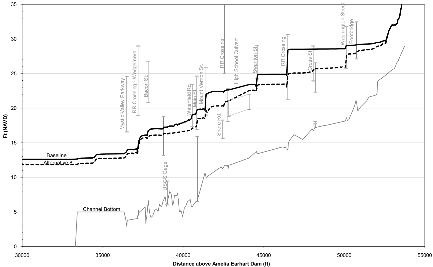
Figure M-2: 100-Year Flood Profile, Alternative 8 vs. Baseline (No Action) Conditions
