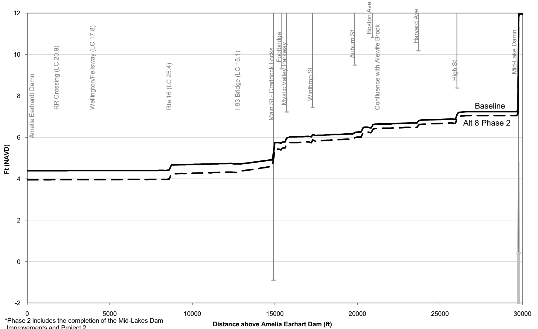
Figure M-12: 100-Year Flood Profile, Alt. 8 Phase 2* vs. Baseline (No Action) Conditions
