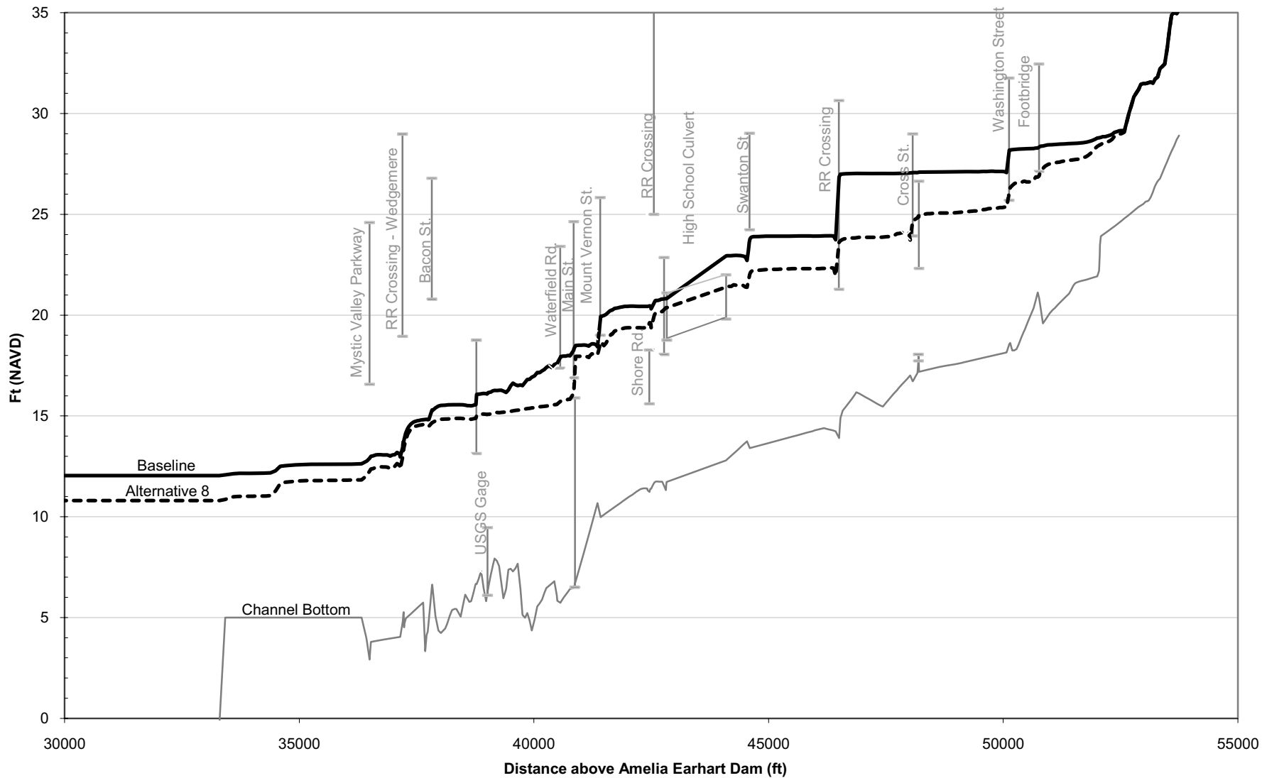
Figure M-5: 50-Year Flood Profile, Alternative 8 vs. Baseline (No Action) Conditions
