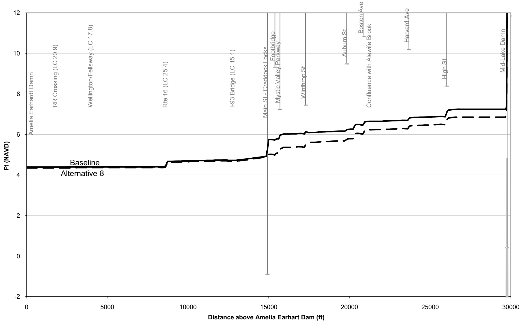
Figure M-3: 100-Year Flood Profile, Alternative 8 vs. Baseline (No Action) Conditions
