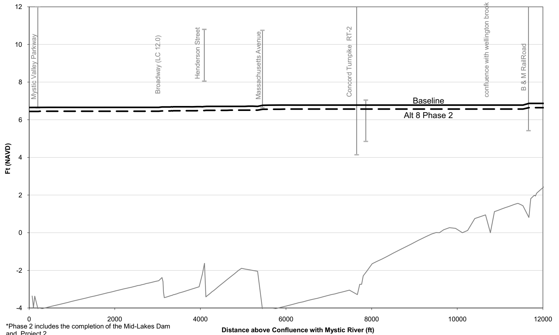
Figure M-13: 100-Year Flood Profile, Alt. 8 Phase 2* vs. Baseline (No Action) Conditions
