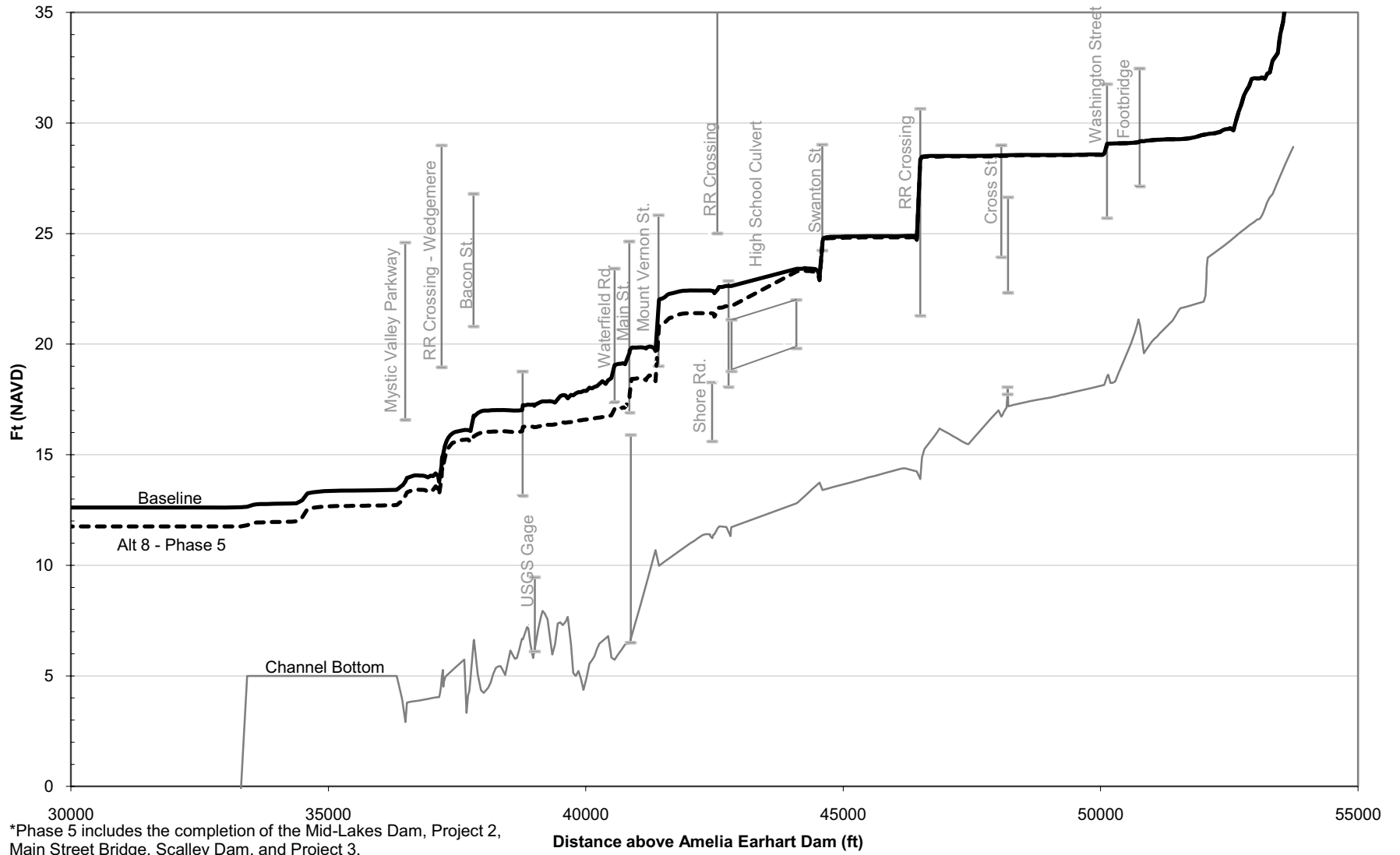
Figure M-20: 100-Year Flood Profile, Alt. 8 Phase 5* vs. Baseline (No Action) Conditions
