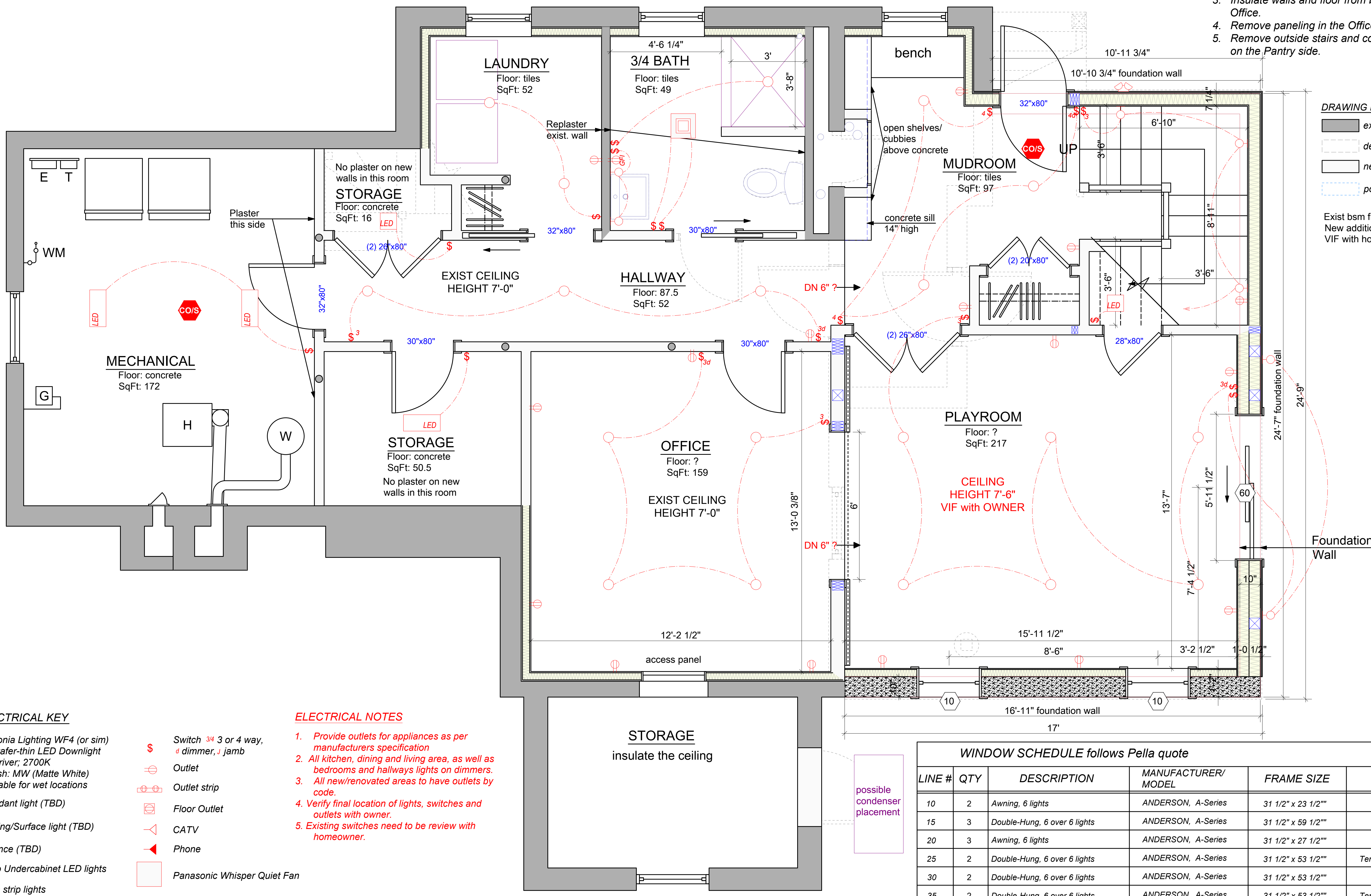
1 Proposed Basement Plan Scale: 1/2" = 1'-0"
